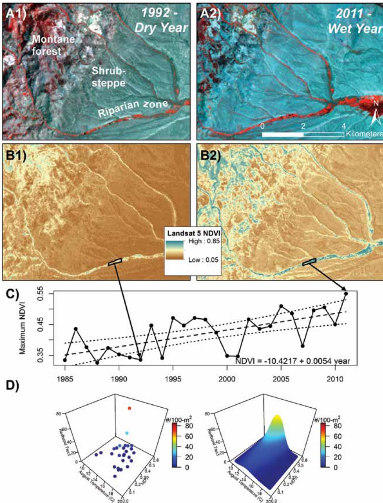
Figure 3. (A) Landsat 5 Thematic Mapper false-color images and (B) NDVI for dry (1992) and wet (2011) years showing interannual differences in riparian vegetation productivity during mid-July in upper Salmon Falls Creek watershed, Nevada. (C) Landsat NDVI significantly increased ( P < 0.001 ) from 1985 to 2011 in a riparian enclosure in the watershed. (D) Redband Trout Oncorhynchus mykiss gairdneri have higher densities at stream sites with higher riparian NAIP NDVI values in Salmon Falls Creek where stream temperatures are suitable as shown by quantile regression.
