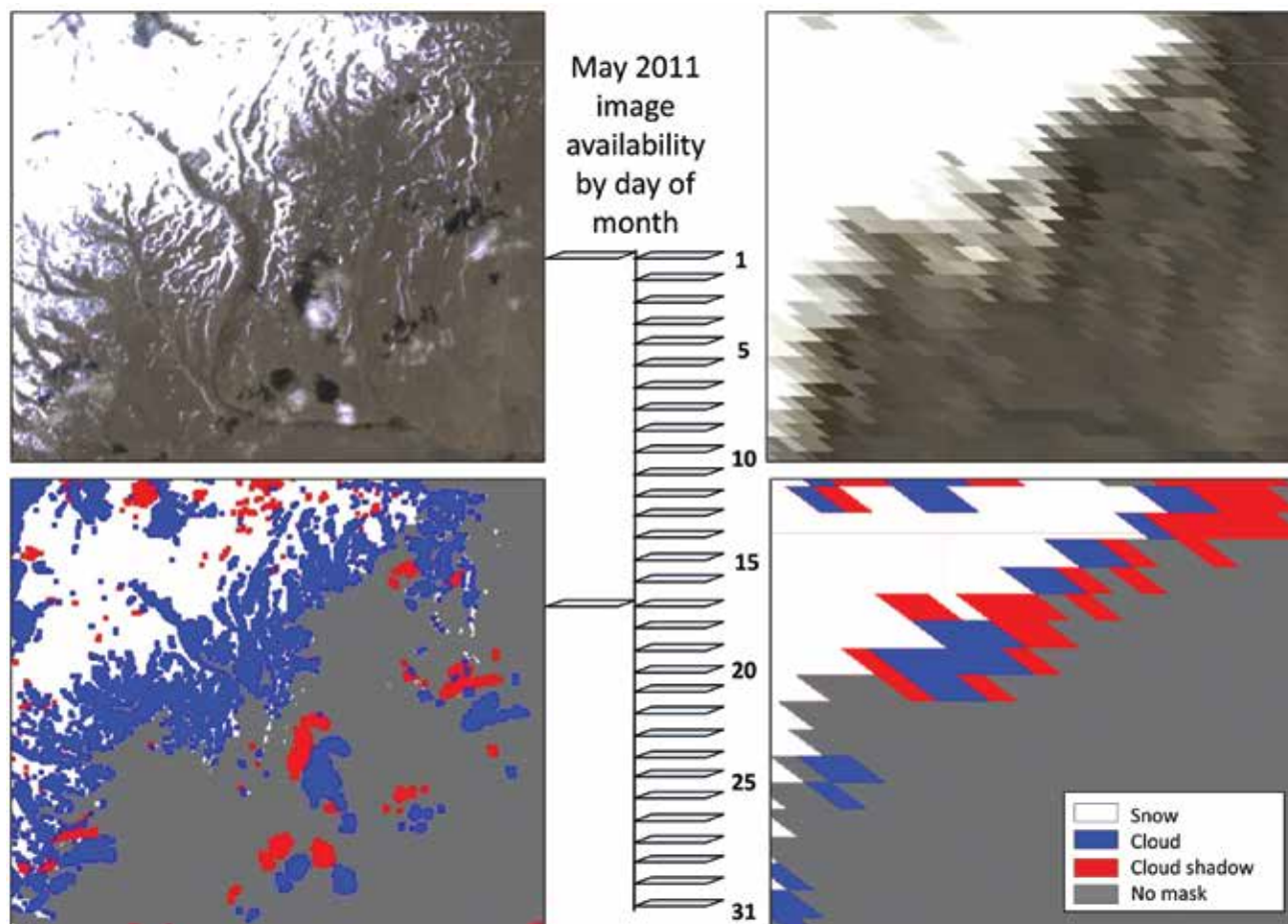
Figure 2. Contrast of spatial and temporal resolution of Landsat 5 Thematic Mapper (left panel: 30-m spatial and ~16-day temporal resolutions) and Terra Moderate Resolution Imaging Spectroradiometer (right panel: 500-m spatial and 1-day temporal resolutions) imagery during May 1, 2011, in upper Salmon Falls Creek watershed, Nevada. Top panels show surface reflectance formatted as natural color images. Bottom panels show derived snow cover data products; bottom left panel is the Landsat image processed using the Fmask algorithm, and bottom right panel is Terra-MODIS based NASA/USGS Land Processes Distributed Active Archive Center 1-km resolution Science Data Set. Note that cloud cover and cloud shadows result in unusable snow cover data (invalid observations) in both data products. Both images were accessed and processed using Google Earth Engine.
