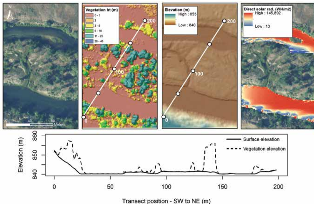
Figure 4. Top panels (left to right): Aerial imagery, airborne LiDAR vegetation height (first laser return minus last laser return) and ground elevation (last laser return), and solar exposure on surface water showing spatial variation in vegetation height (reflecting vegetation type and structure), hillslope and floodplain topography, and stream shading for the Boise River, Boise, Idaho. Bottom panel: Transverse profile of vegetation and floodplain elevations from LiDAR data. LiDAR data resampled to 3-m spatial resolution.
