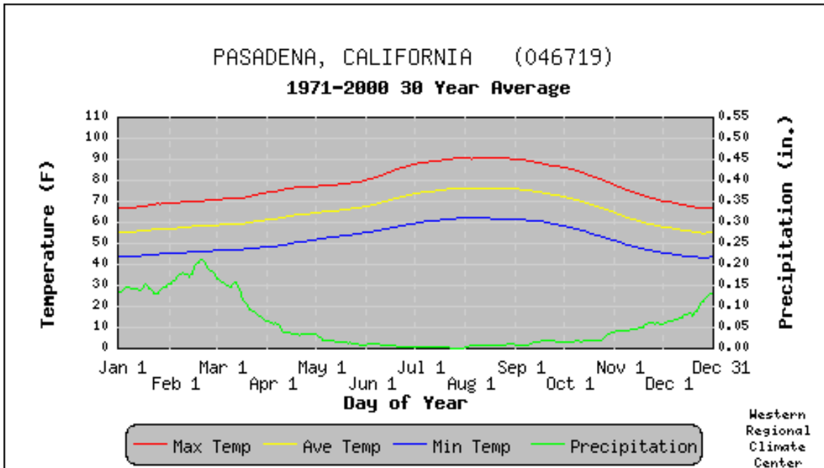
Figure 13 - Pasadena Climate
